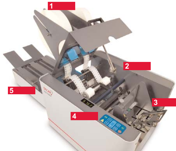
Model 2020 Dual Tabber shown with optional conveyor for improved handling of media.
