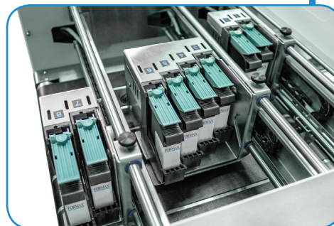
Three independent print heads: 2-pen + 4-pen + 2-pen stitched design
