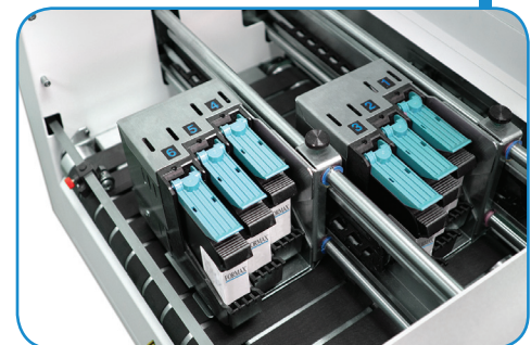
Two independent print heads: 3-pen stitched + 3-pen stitched design
